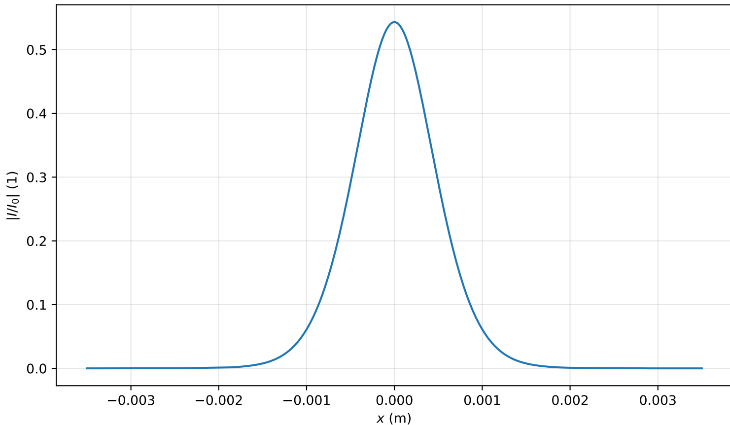
Intensity profile I(x, y = 0, z = 3.105m)/I_0 , P_{in}=0.5P_{cr} , artificial time
